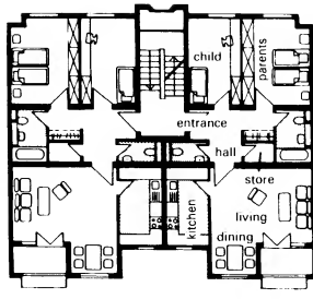
3 Two dwellings per floor
